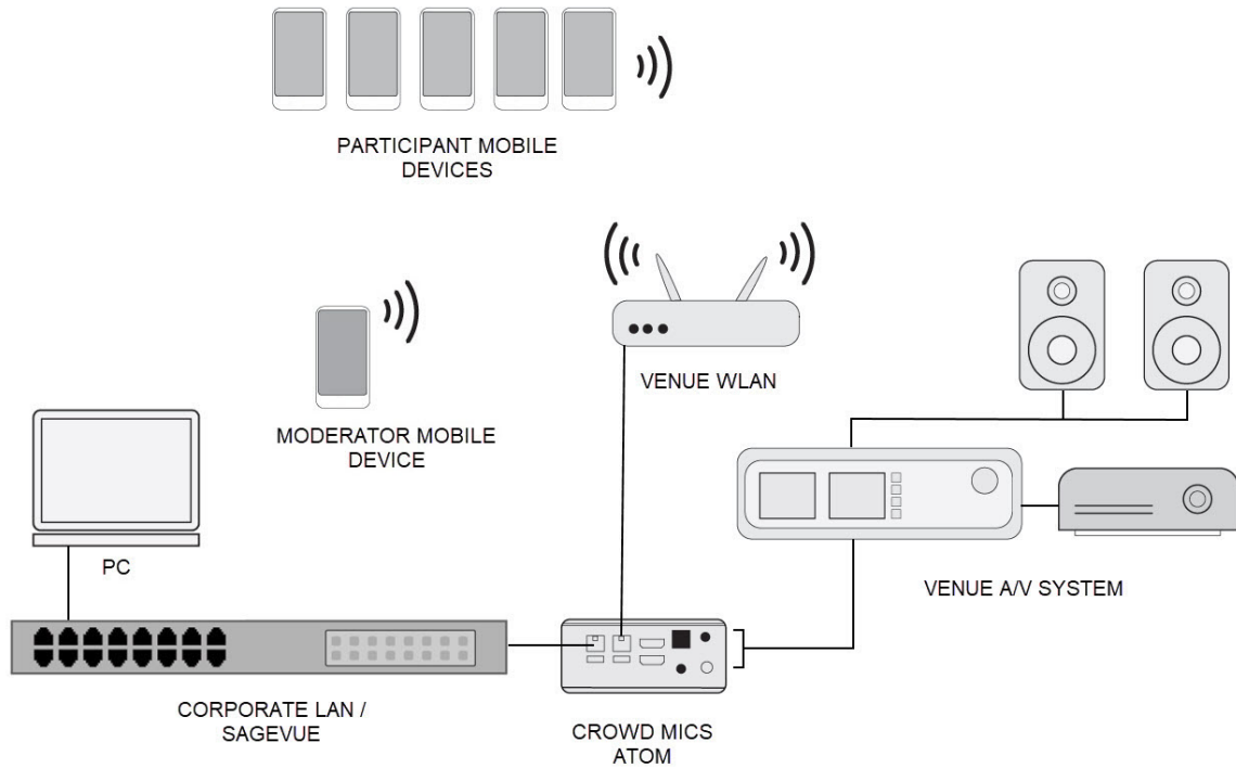
Typical Enterprise Network Connection Diagram
