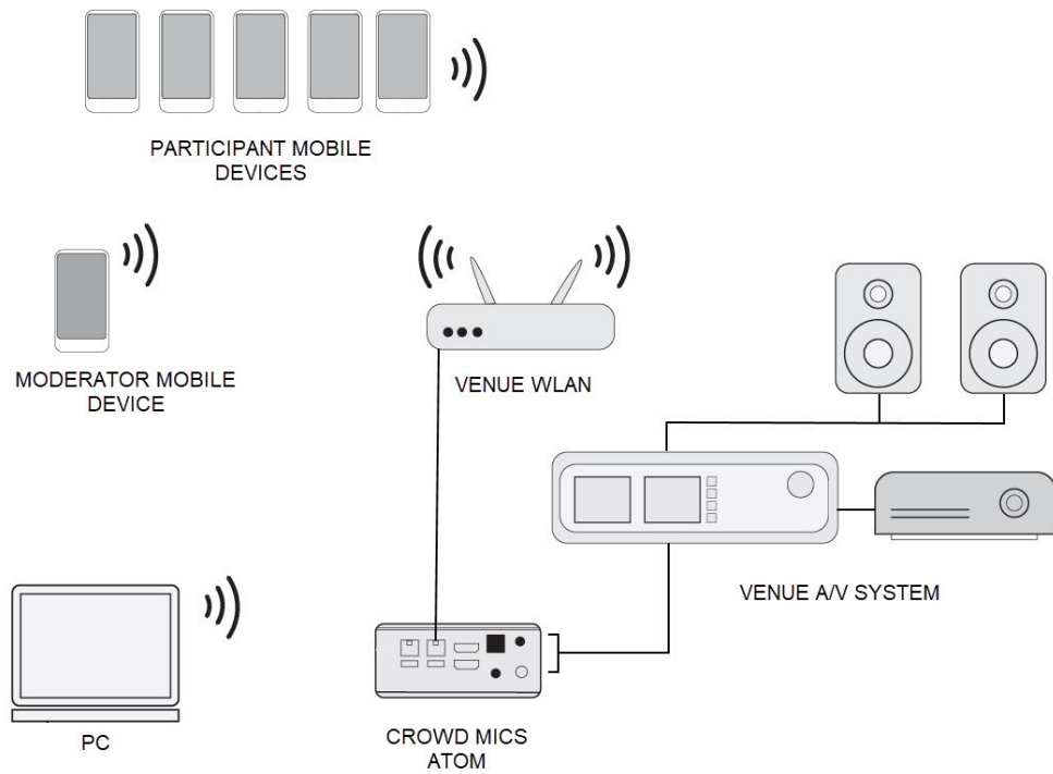
Typical Standalone Network Connection Diagram
